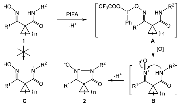
Scheme 2. Plausible Mechanism for the Reaction of Cycloalkyl Oximes 1 with PIFA/TFA
