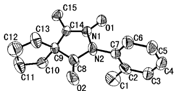
Figure 1. ORTEP drawing of 2l .
